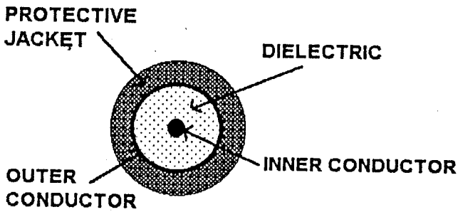
Figure 2. Cross-section of coaxial cable.
