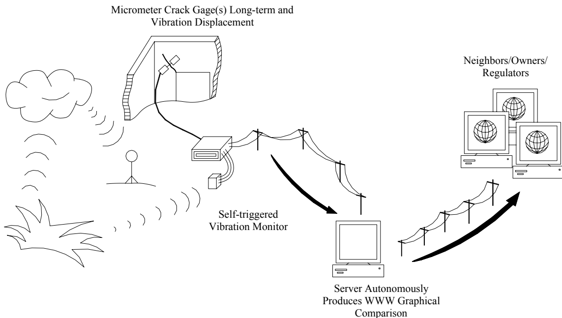
Figure 1 AUTONOMOUS CRACK MEASUREMENT
