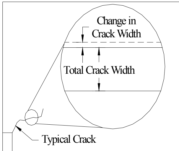
Figure 2 Definition of the change in crack width hereafter called crack displacement.
