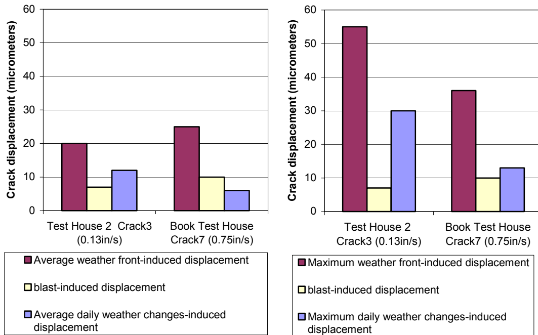
Figure 10 Comparison of Average and Maximum Weather Front and Daily Environmental effects with Those of the Maximum Vibration Effect
