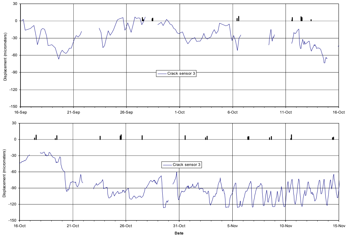
Figure 9: Comparison of Long-Term and Vibratory Response of Crack 3
