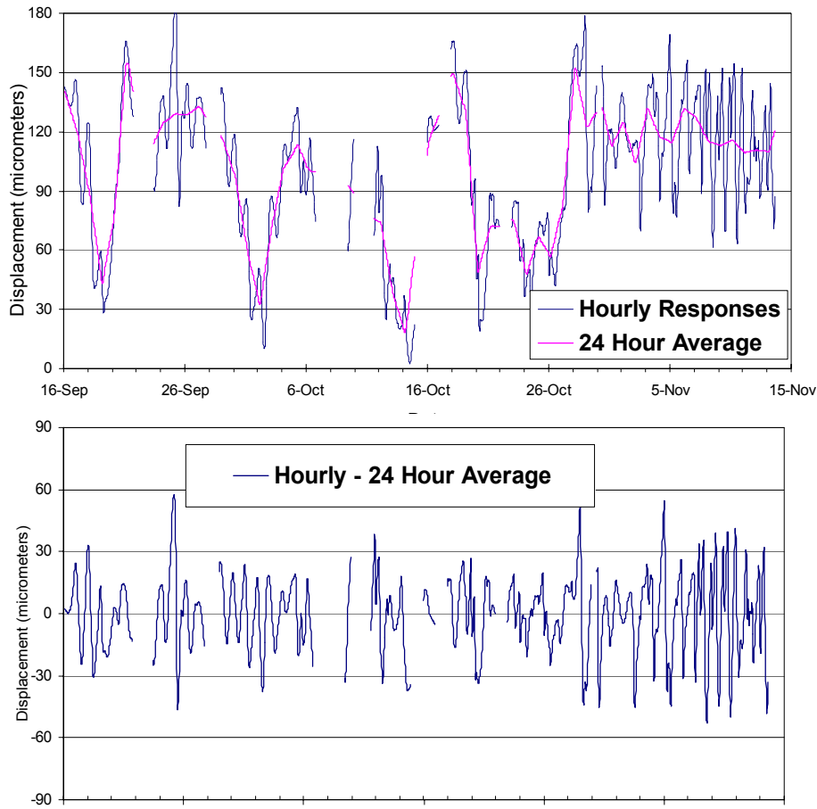
Figure 8: Comparison of Crack Response to Weather Front and Daily Environmental Effects.
