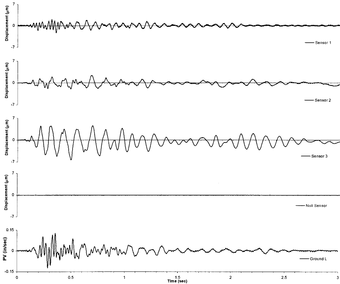
Figure 7 Time histories crack response and ground motion response for blast event oct0-13 for comparison of dynamic response of null sensor
