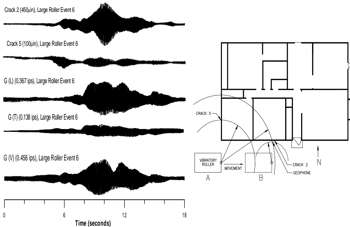
Figure 3 Time Histories of Crack Displacement and Ground (Particle) Velocity Produced by Vibratory Roller Compaction within 3 m of the House
