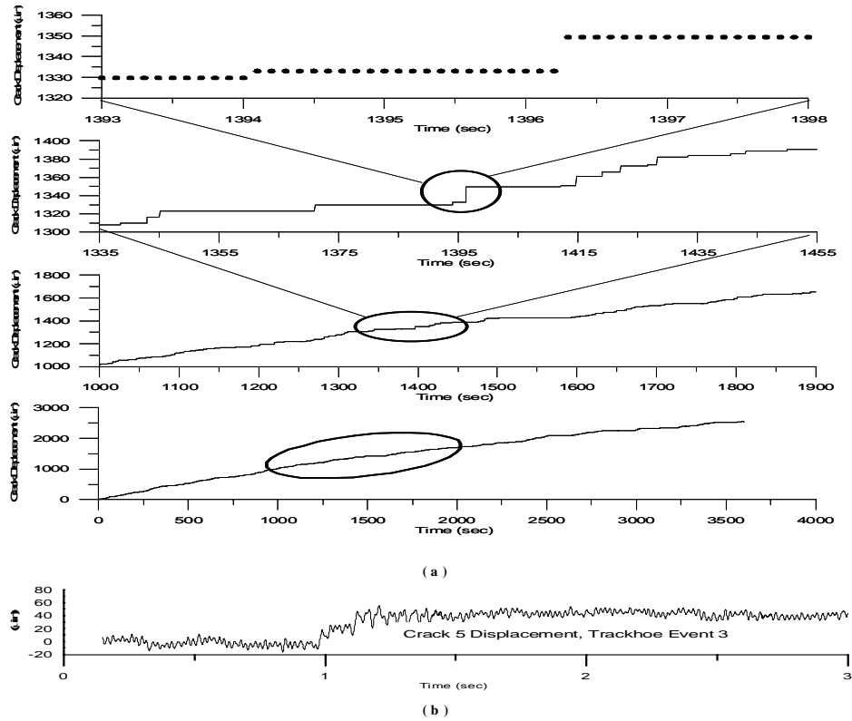
Figure 6 Stick-Slip Behavior of Crack Displacement and Potential Misinterpretation of Effect of Vibratory Crack Response
