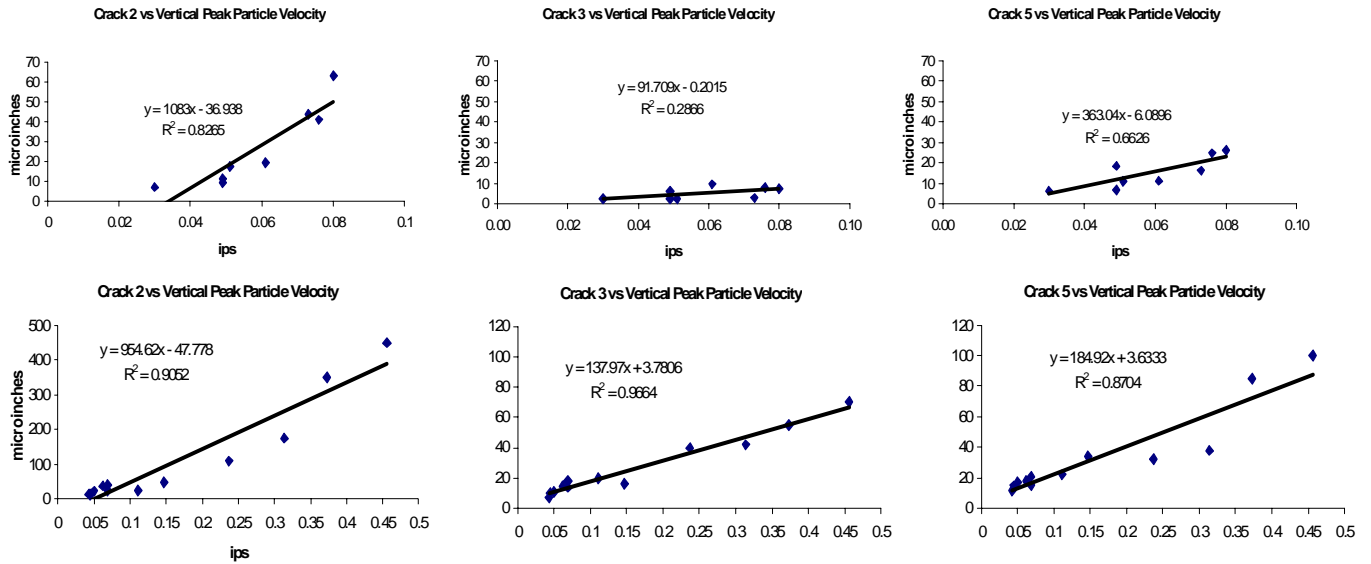
Figure 7 Correlation of Crack Displacement in micro inches (y axis) with Peak Particle Velocity (ips) (1 ips = 25 mm/s) (x axis) for Cracks 2, 3 & 5 for Trackhoe (top row) and Vibratory Roller Excitation (bottom row)
